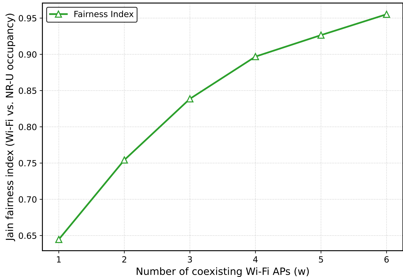
Wi-Fi/NR-U Coexistence Fairness
