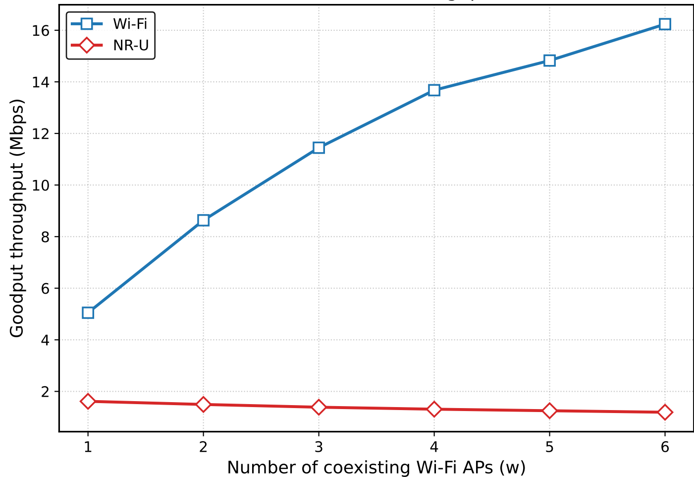
Wi-Fi vs. NR-U: Throughput
