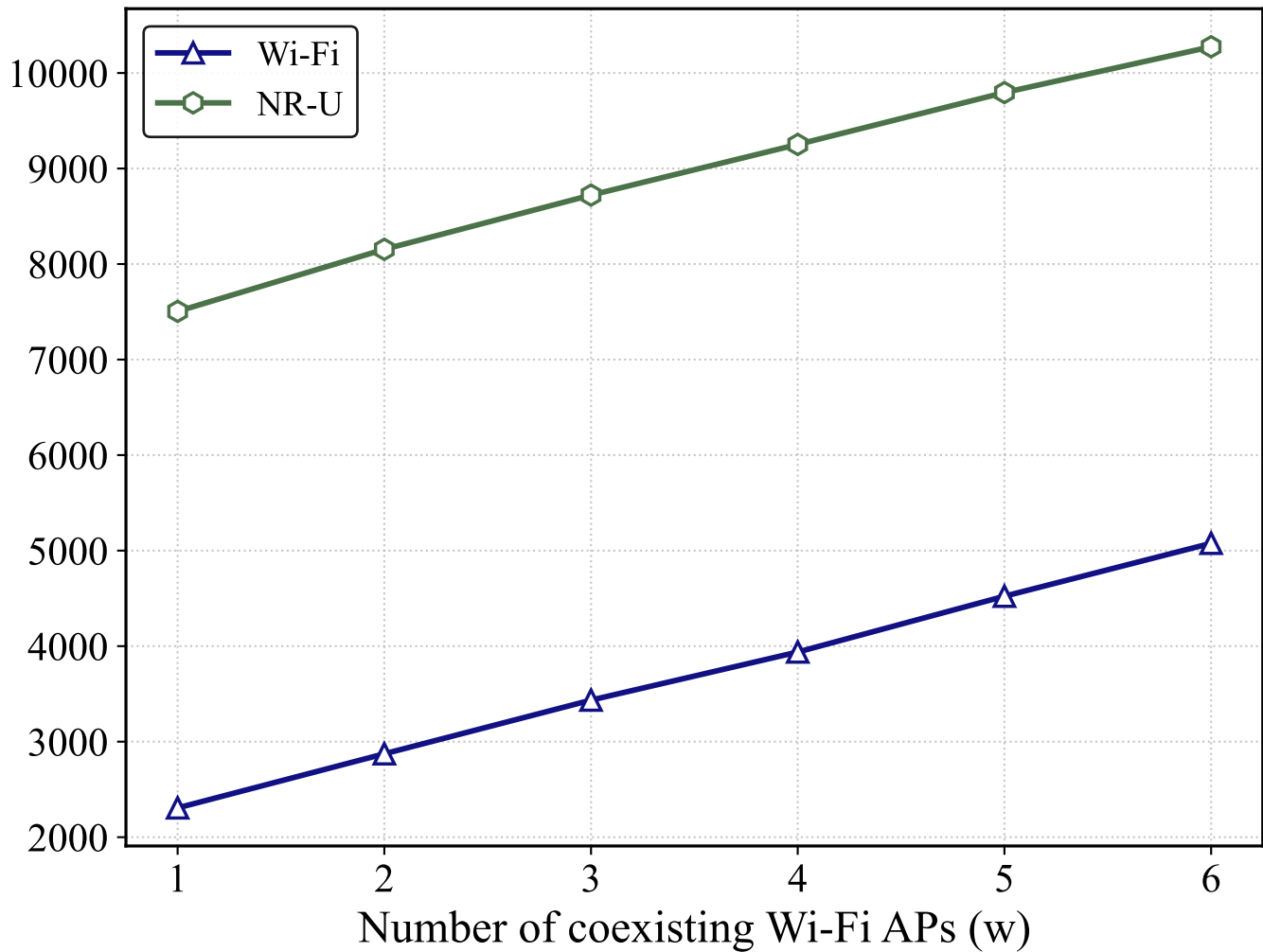
Average packet delay ( \mu\text{s} )
