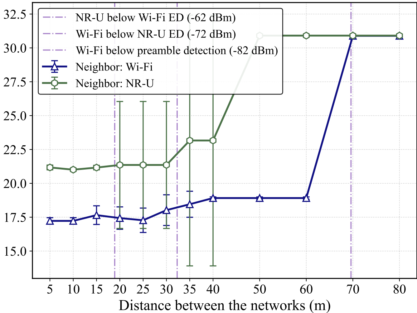
Network A throughput (Mbps)
