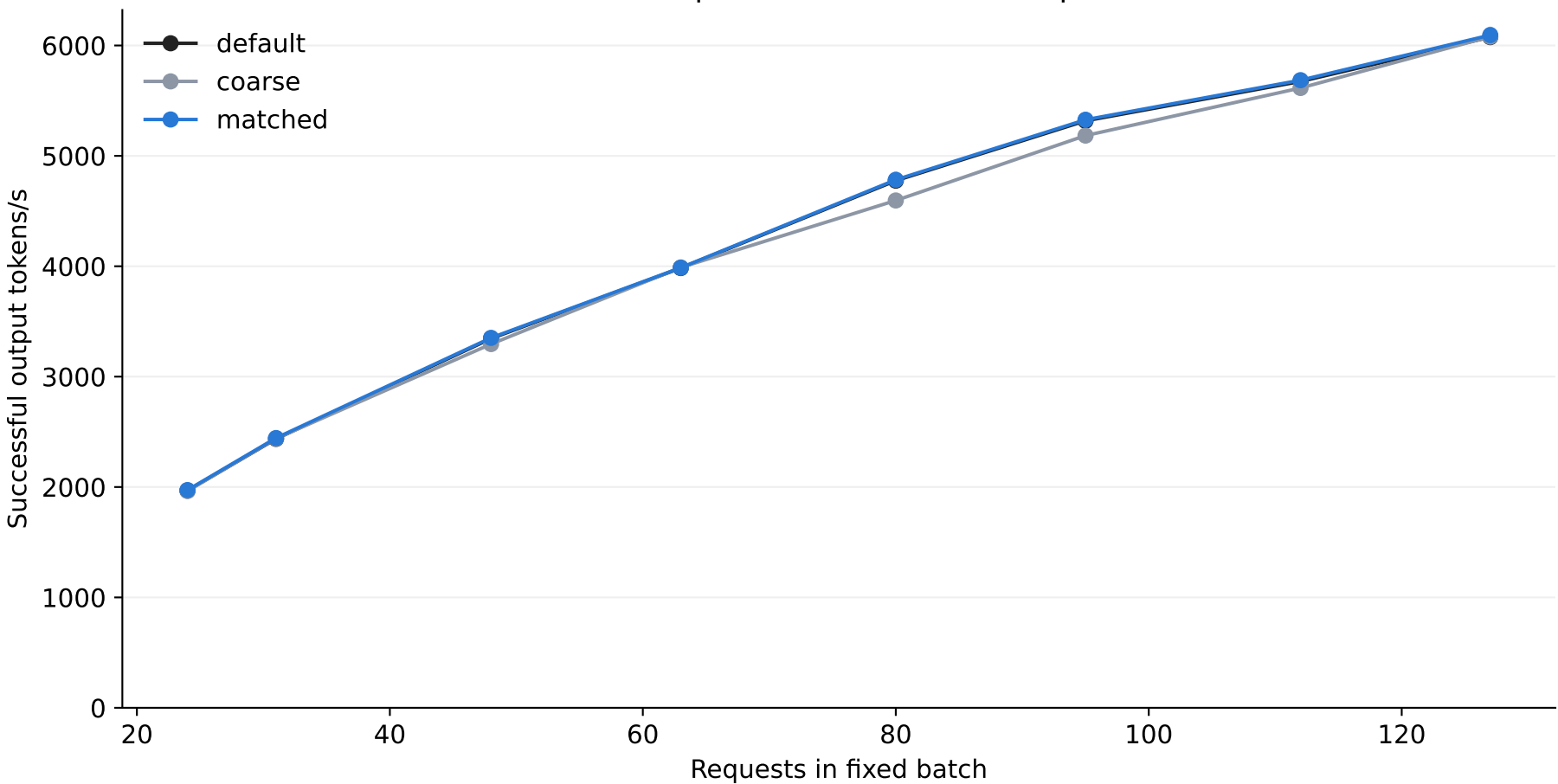
CUDA-graph configuration sensitivity Points: measured repetitions · Lines: within-process means
