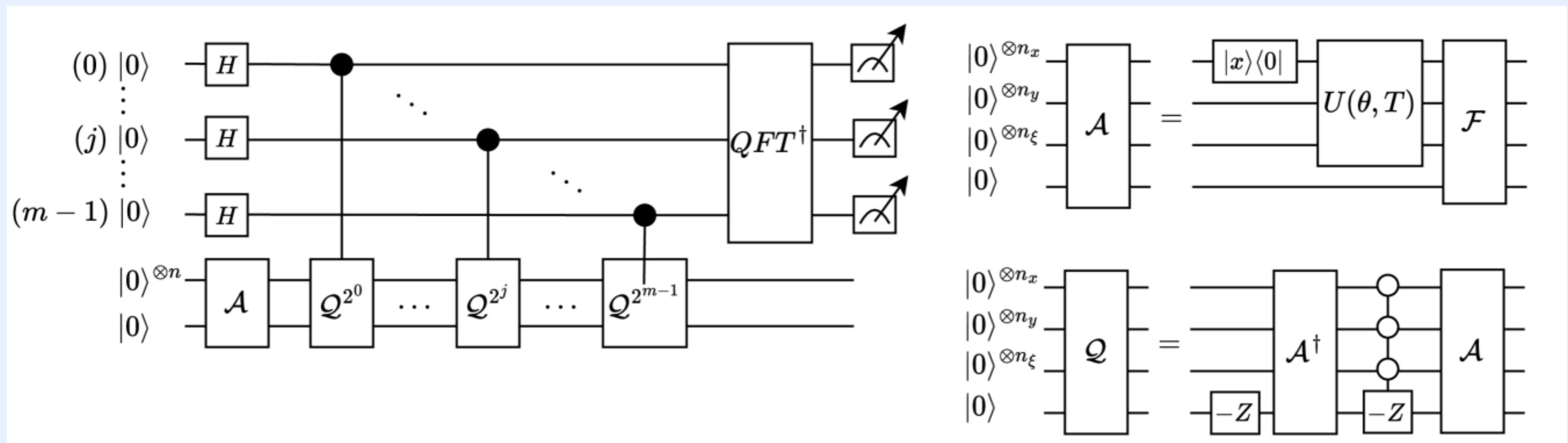
Fig. 2 [1]: QAE circuit. A = F \cdot U(\theta, T) ; Q is the Grover iterate.
