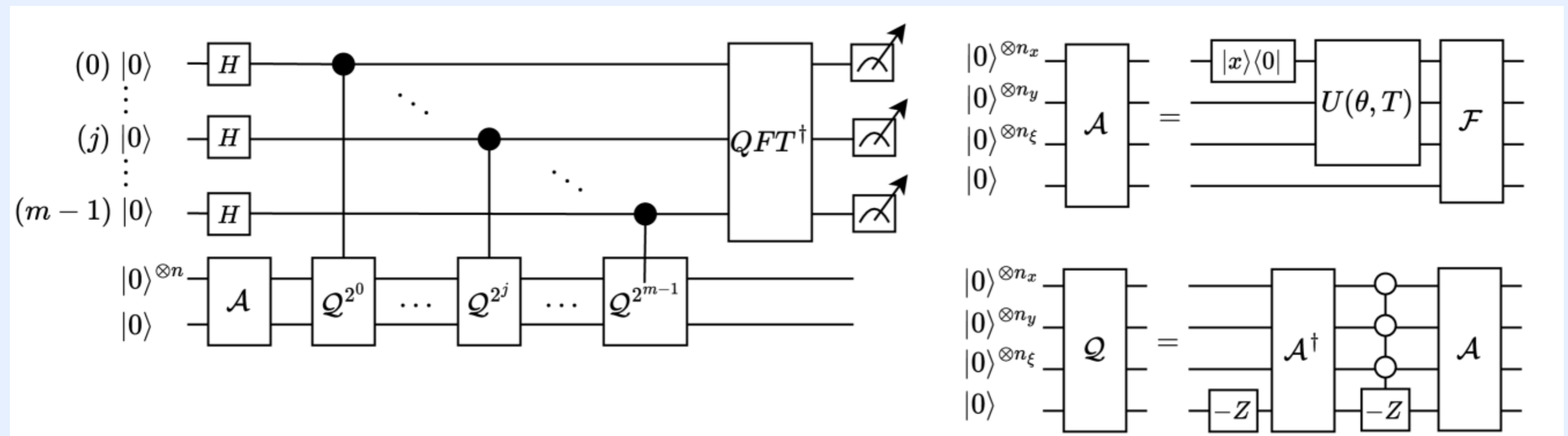
Fig. 2 [1]: QAE circuit. A = \mathcal{F} \cdot U(\theta, T) ; Q is the Grover iterate.
