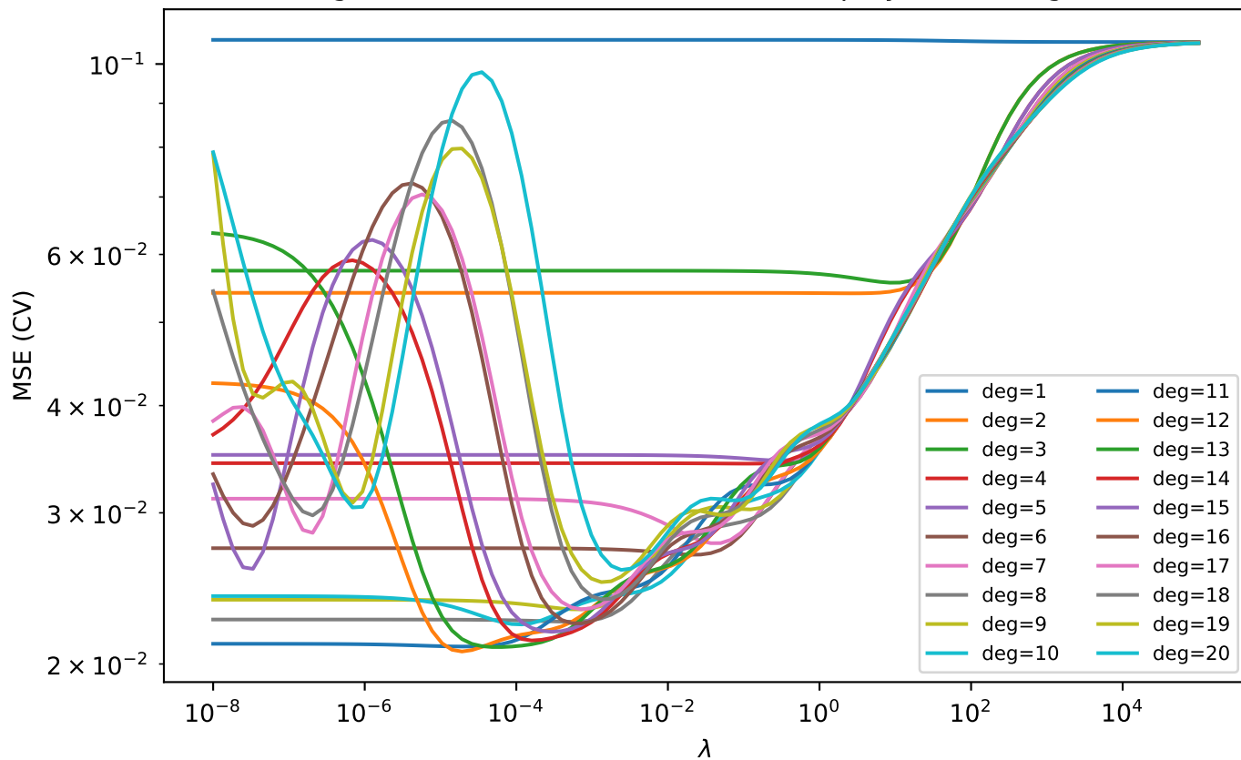
Ridge CV-MSE vs lambda for different polynomial degrees
