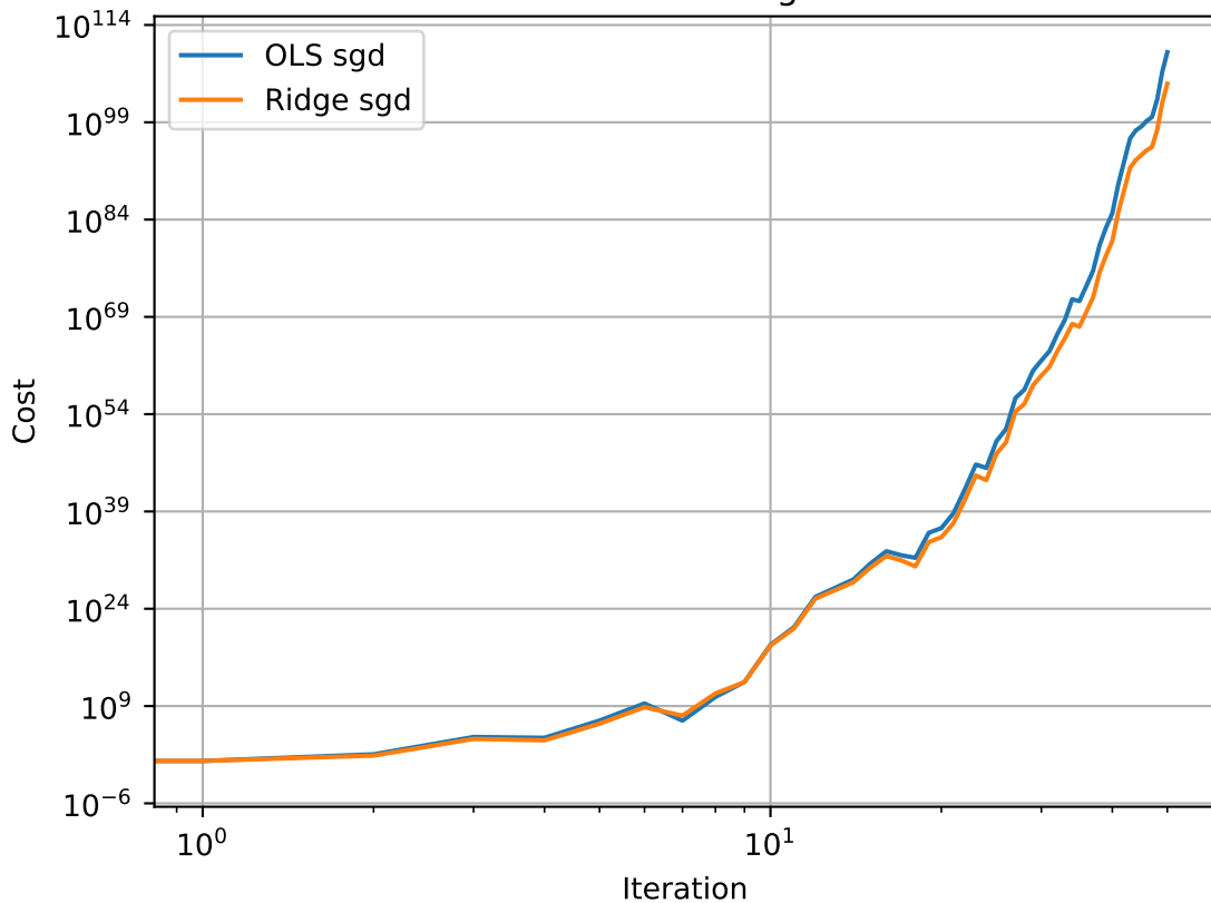
Cost function of stochastic gradient descent
