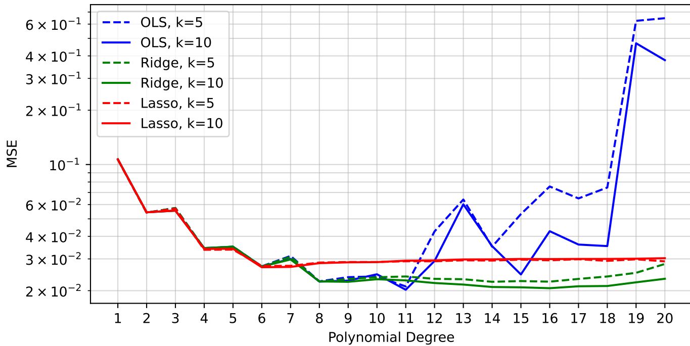
Mean squared error comparison different methods, \lambda = 0.001
