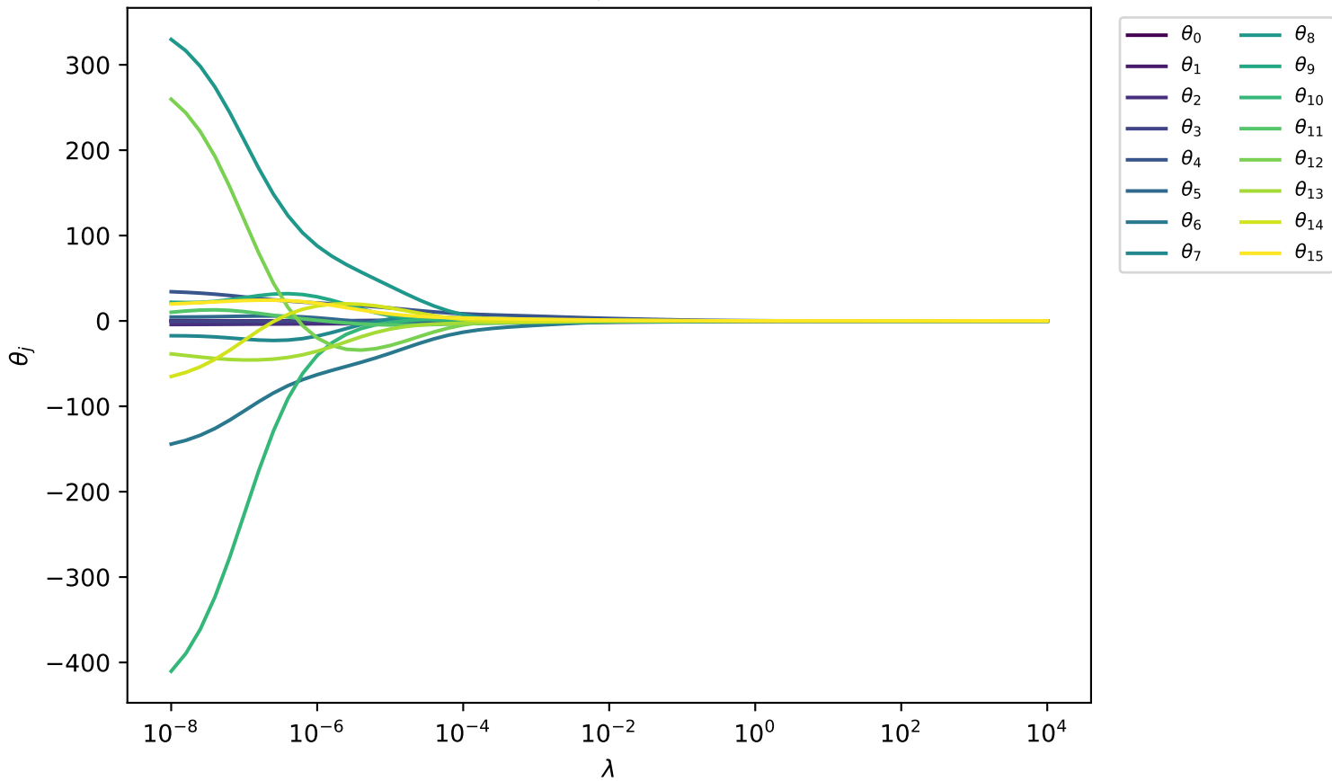
Ridge coefficients \theta_j over \lambda at degree 15
