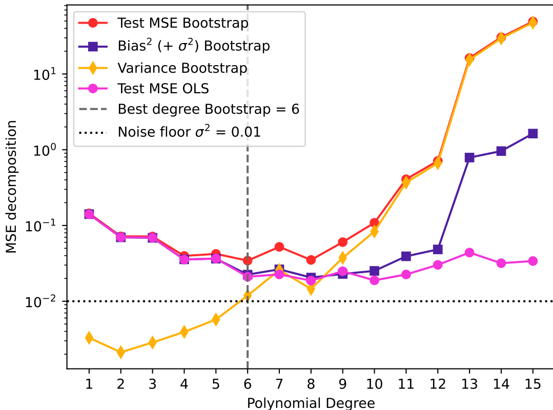
Bias-variance tradeoff and test MSE for OLS seed = i + 2026
