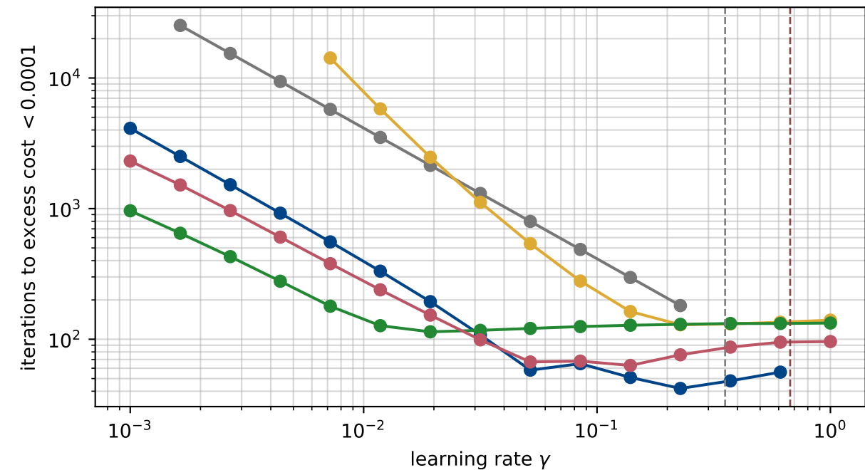
Needed iterations for convergence of different machine learning methods based on learning rates
