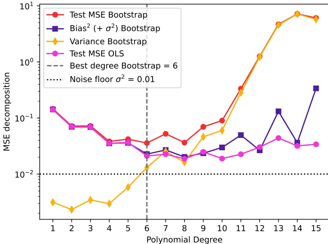
Bias-variance tradeoff and test MSE for OLS seed = i + 42
