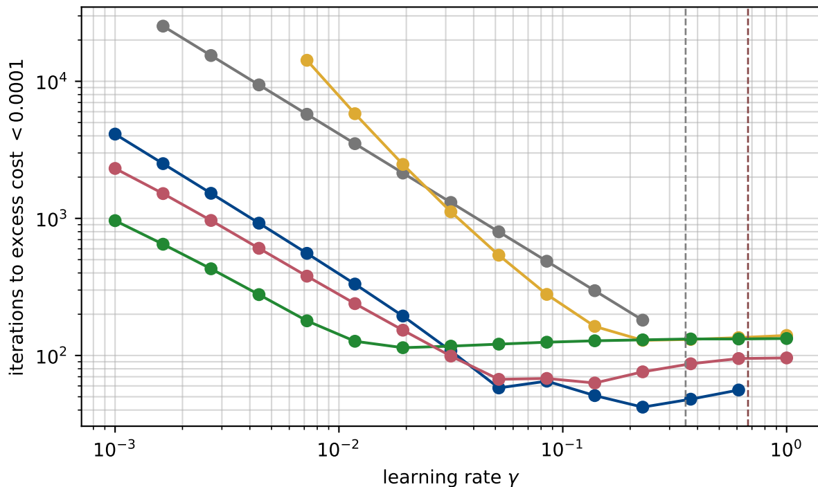
Needed iterations for convergence for learning rates
