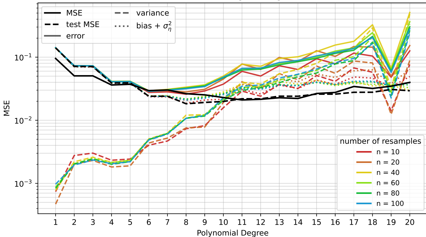
Comparing n refits with bootstrap on Ridge with 5 folds using training data
