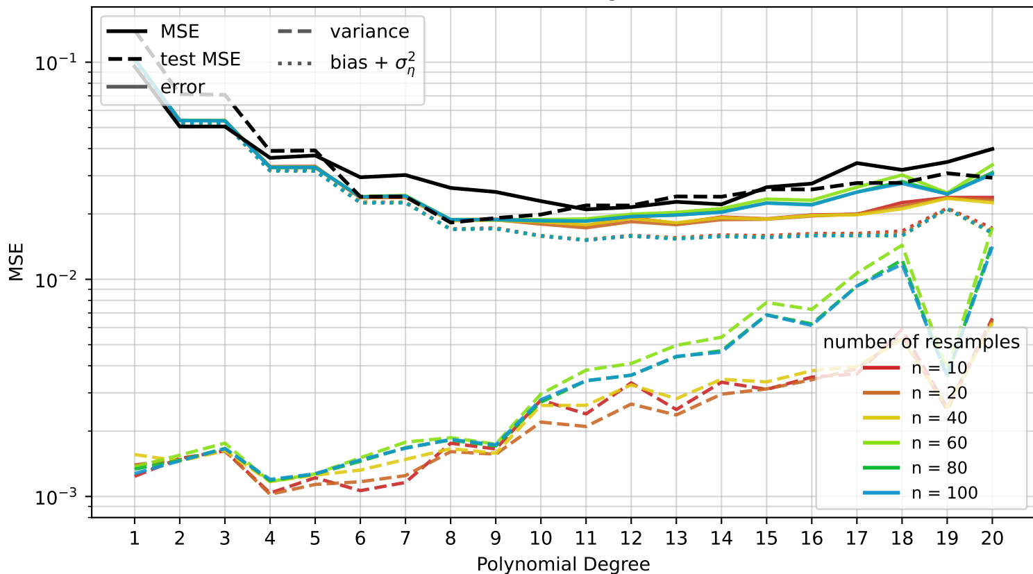
Comparing n refits with bootstrap on Ridge with 5 folds using all data
