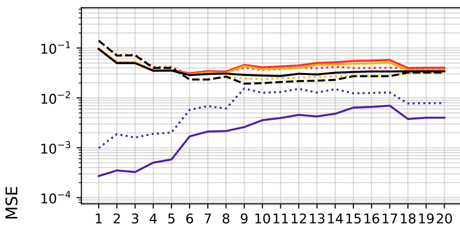
Ridge k = 10
