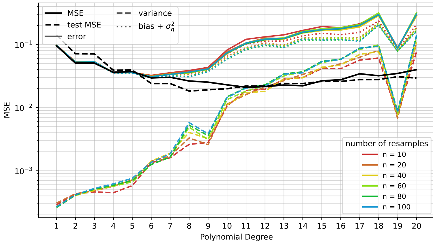
Comparing n refits with kfold on Ridge with 5 folds using training data
