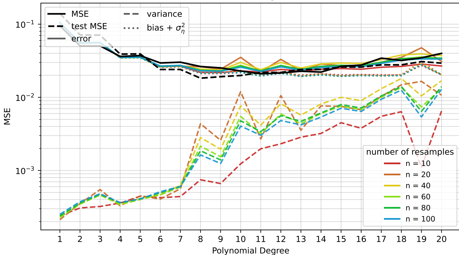
Comparing n refits with kfold on Ridge with 5 folds using all data
