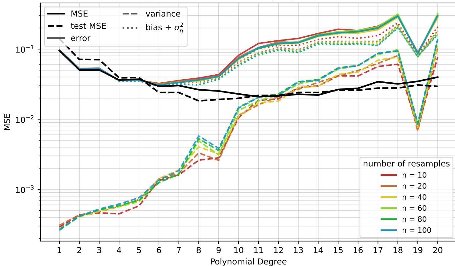
Comparing n refits with kfold resampling on Ridge with 5 folds
