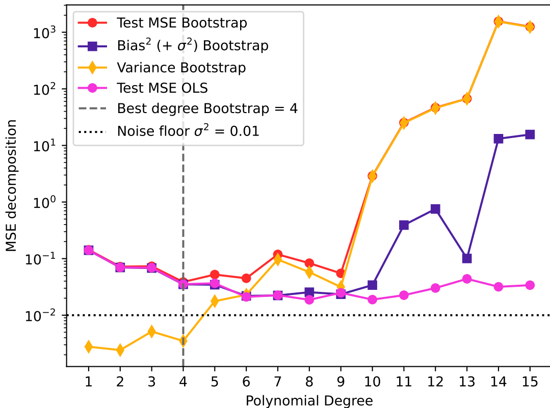
Bias-variance tradeoff and test MSE for OLS seed = i + 500
