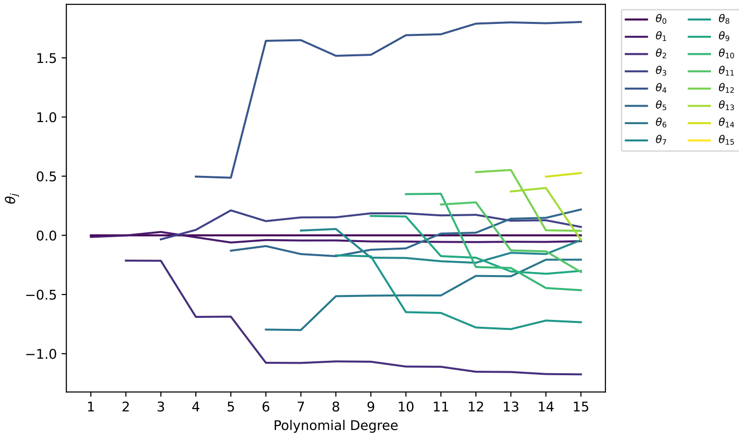
Coefficients of \theta_j for Ridge over polynomial degree
