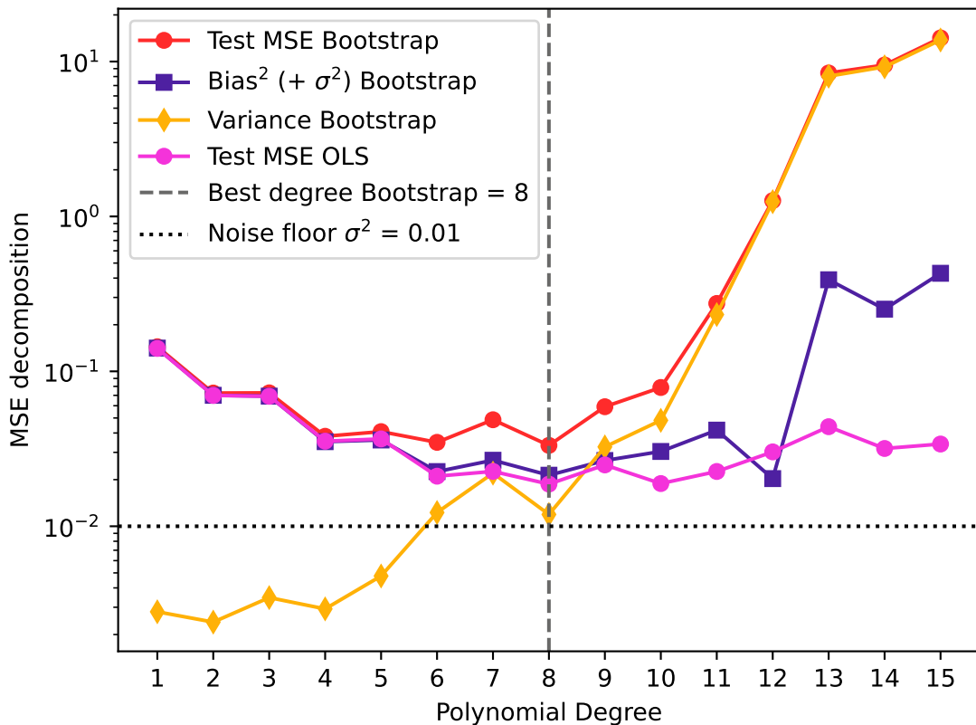
Bias-variance tradeoff and test MSE for OLS
