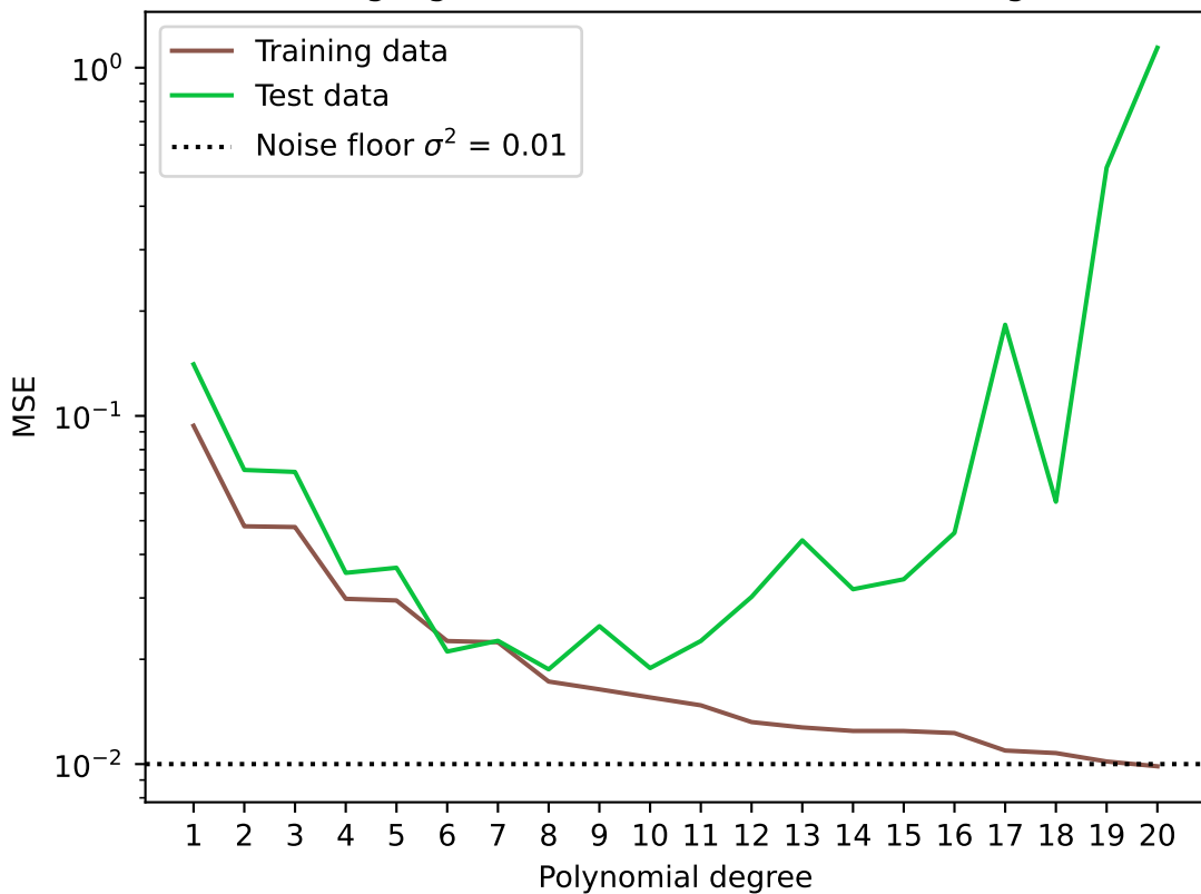
Recreating Figure 2.11 with MSE from OLS Regression
