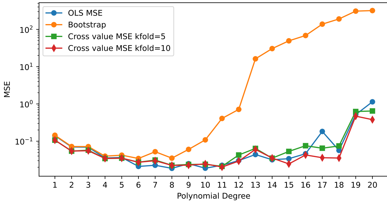
Mean squared error comparison different methods
