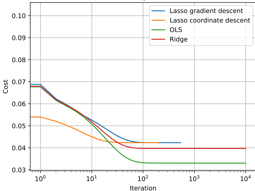
Cost function of gradient descent
