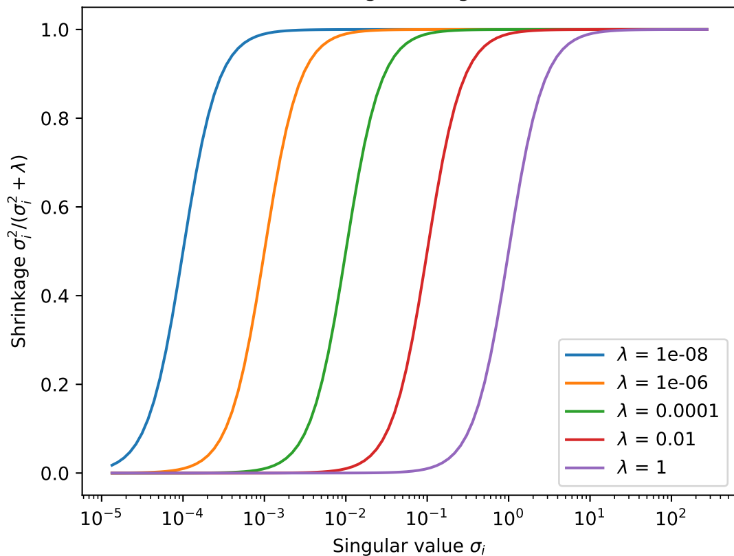
Shrinkage through SVD
