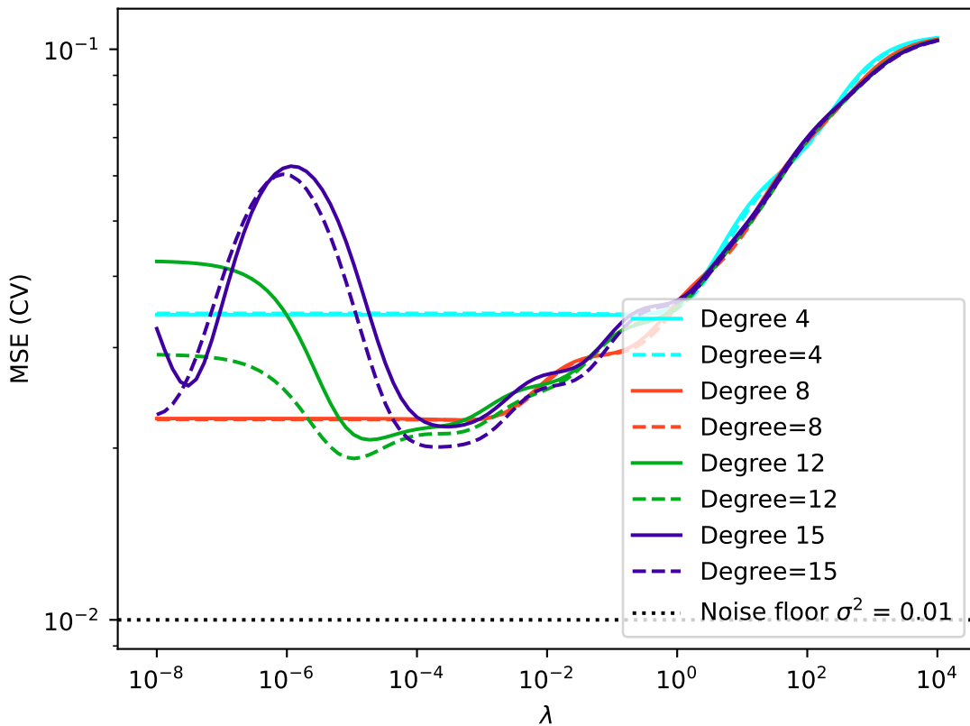
Ridge CV-MSE over \lambda s. k = 5 (solid) and k = 10 (dashed)
