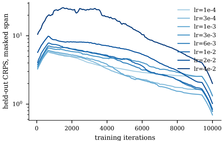
Patched Transformer 3.32M small architecture: LR sweep
