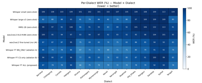
Fig. 5: Model × dialect WER heatmap. Darker is higher WER.
