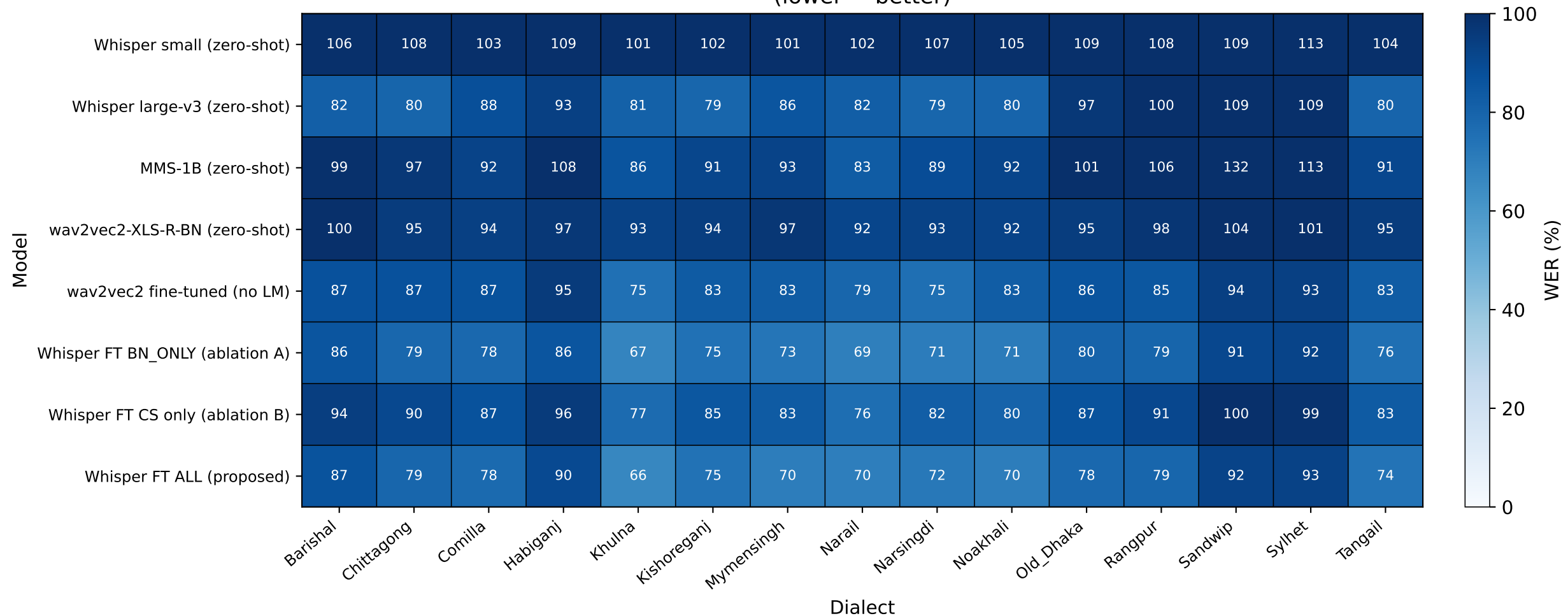
Per-Dialect WER (%) — Model × Dialect (lower = better)
