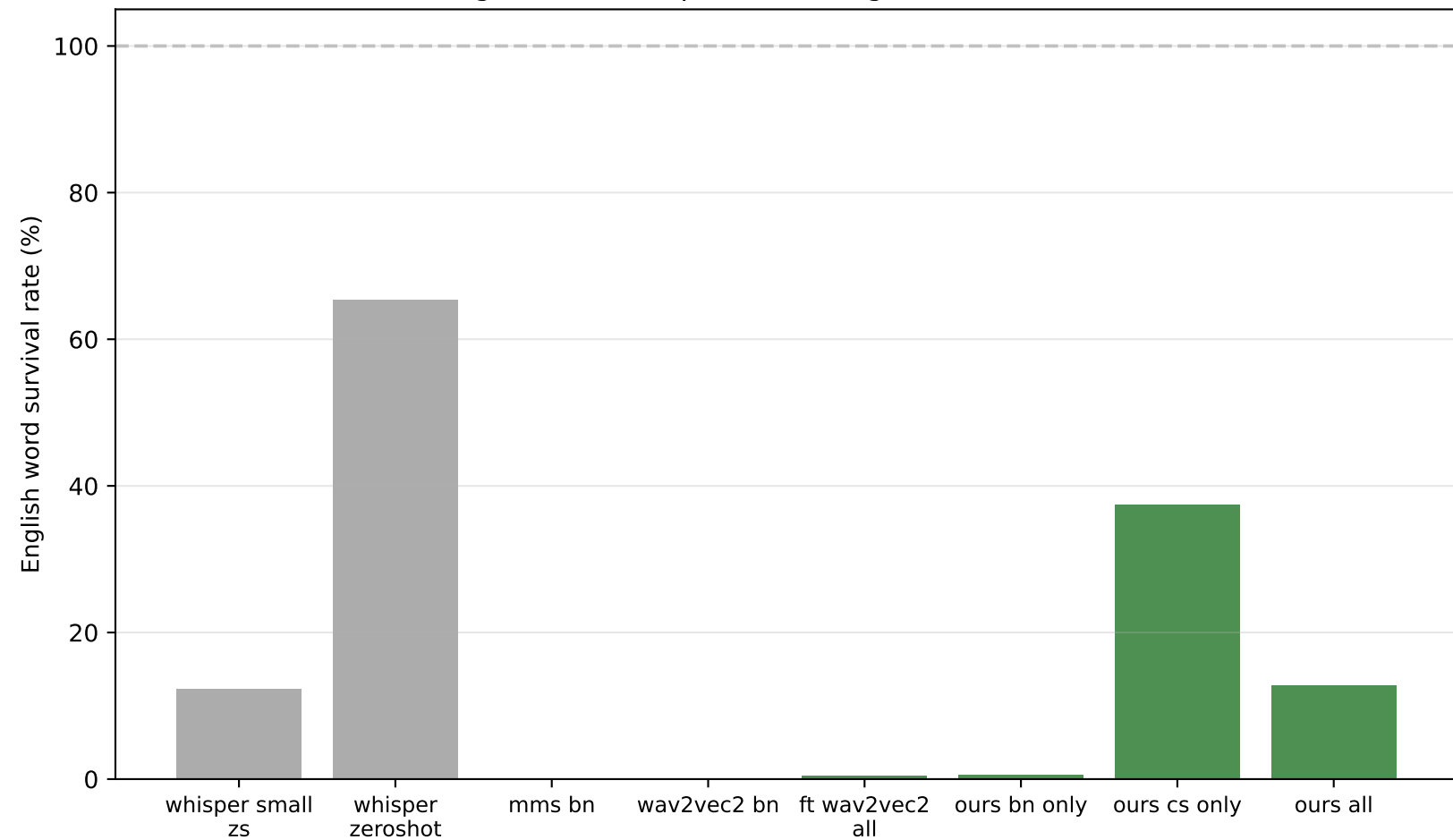
English CS Word Survival Rate (higher = model preserves English words better)
