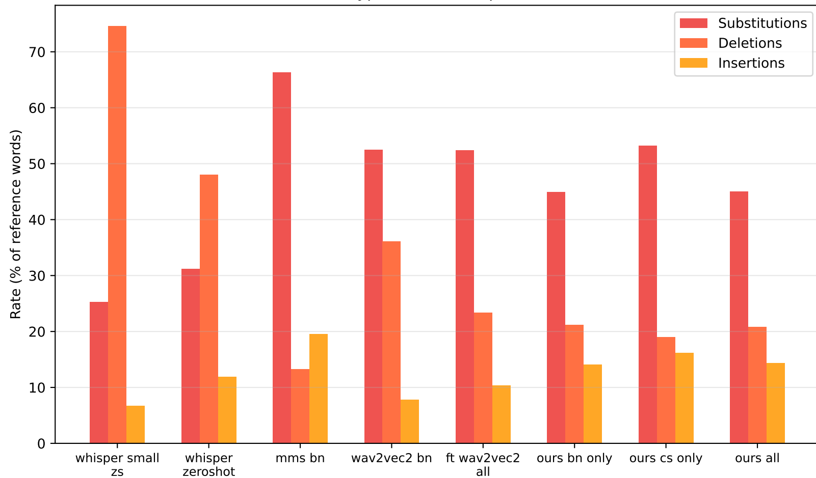
Error Type Breakdown per Model
