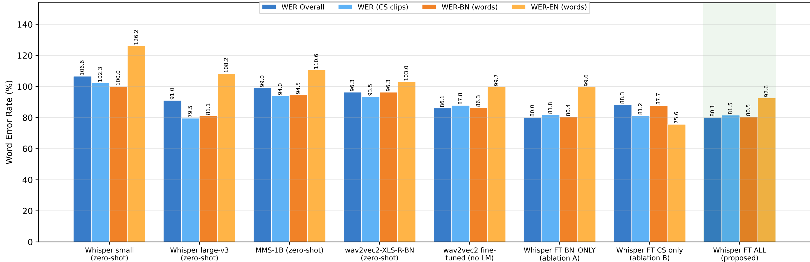
ASR Performance: WER Comparison Across Models (Bengali Dialect + Code-Switching Test Set)
