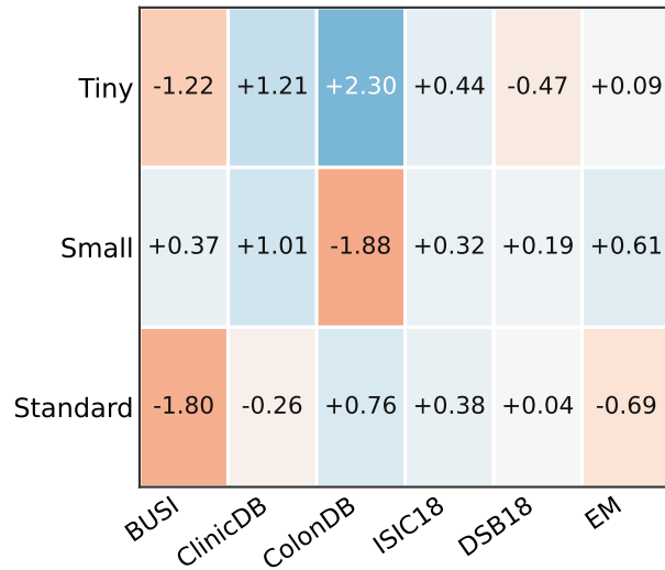
Adaptive soft
