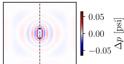
Residual ( r = 10 ) Max \Delta : 0.06 psi
