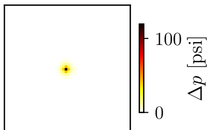
POD ( r = 10 ) \varepsilon_G = 0.0001\%
