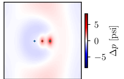
BDF t = 16245 hr Residual Max \Delta : 8.30 psi
