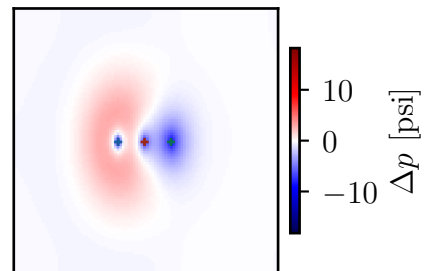
Buildup t = 22044 hr Residual Max \Delta : 18.19 psi
