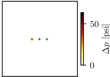
W1 alone t = 12 hr POD r = 4 \varepsilon_G = 0.0085\%
