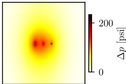
BDF t = 16245 hr POD r = 4 \varepsilon_G = 0.0081\%
