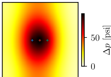
Buildup t = 22044 hr POD r = 4 \varepsilon_G = 0.0225\%
