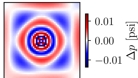
Residual ( r = 10 ) Max \Delta : 0.01 psi
