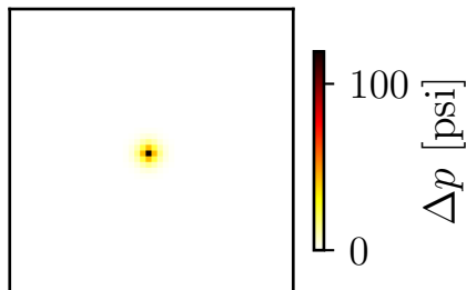
Ground Truth t = 9.0 hr
