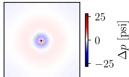
Residual ( r = 3 ) Max \Delta : 28.18 psi
