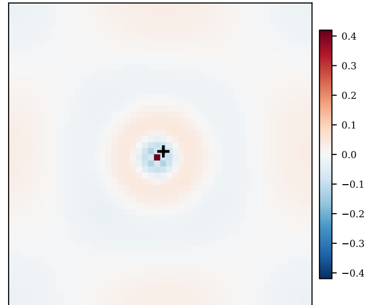
u_7 \quad \sigma_7/\sigma_1 = 4.7e-04
