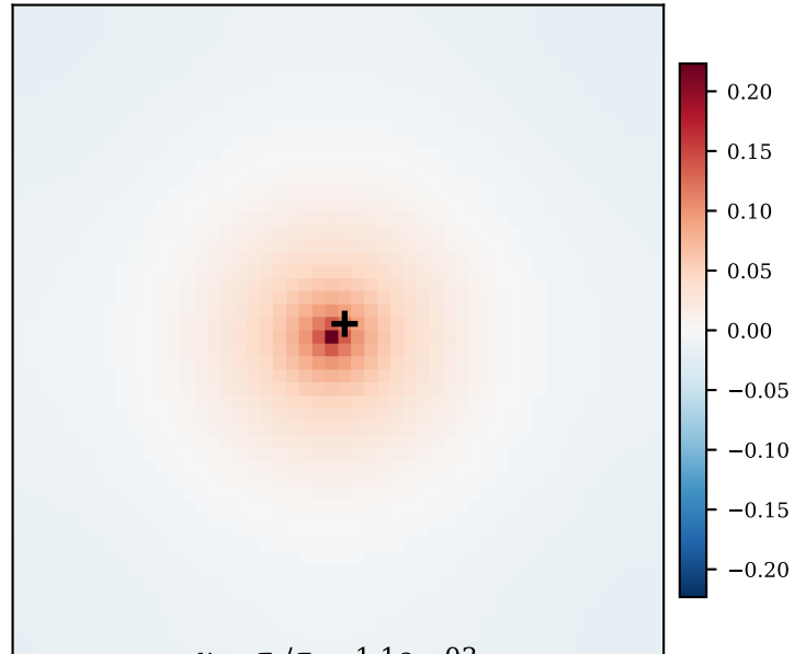
u_6 \quad \sigma_6/\sigma_1 = 1.1e-03
