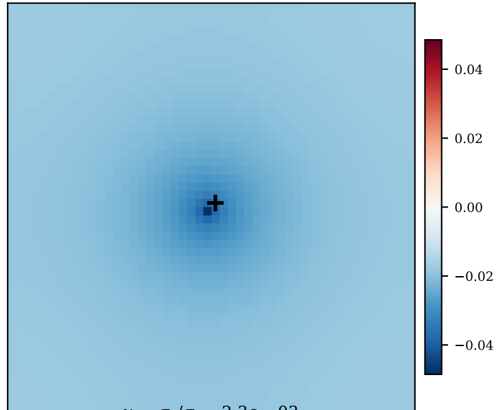
u_5 \quad \sigma_5/\sigma_1 = 2.3e-03
