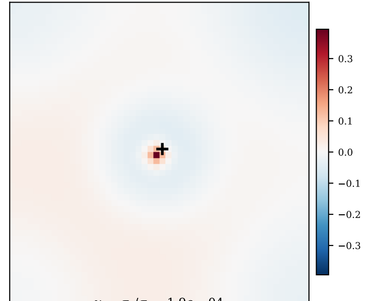
u_8 \quad \sigma_8/\sigma_1 = 1.9e-04
