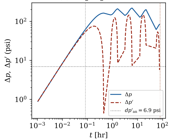
(b) Log-log Bourdet
