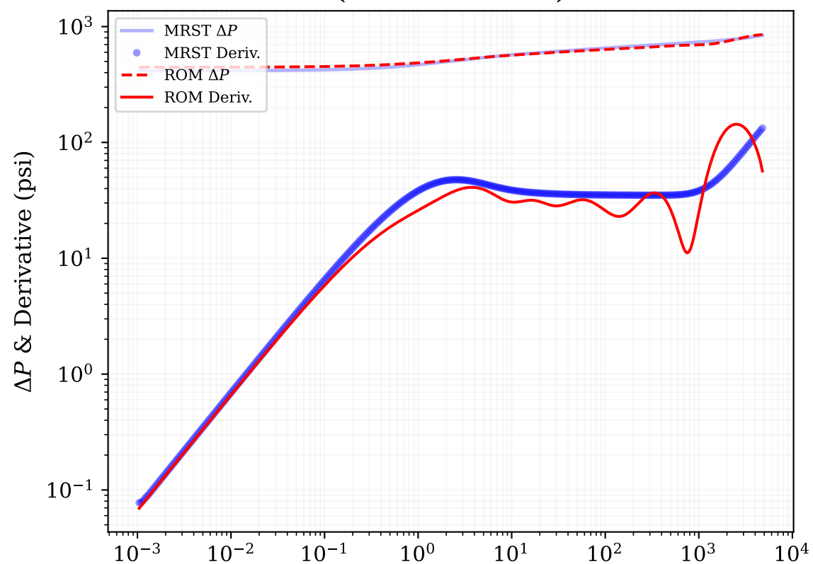
Case: k070_s05_sched1 (Rel. Error: 2.49e-02)
