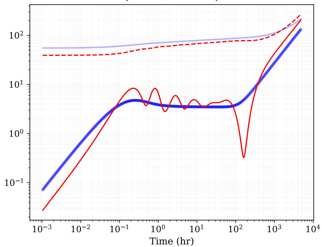
Case: k150_s04_sched1 (Rel. Error: 3.46e-03)
