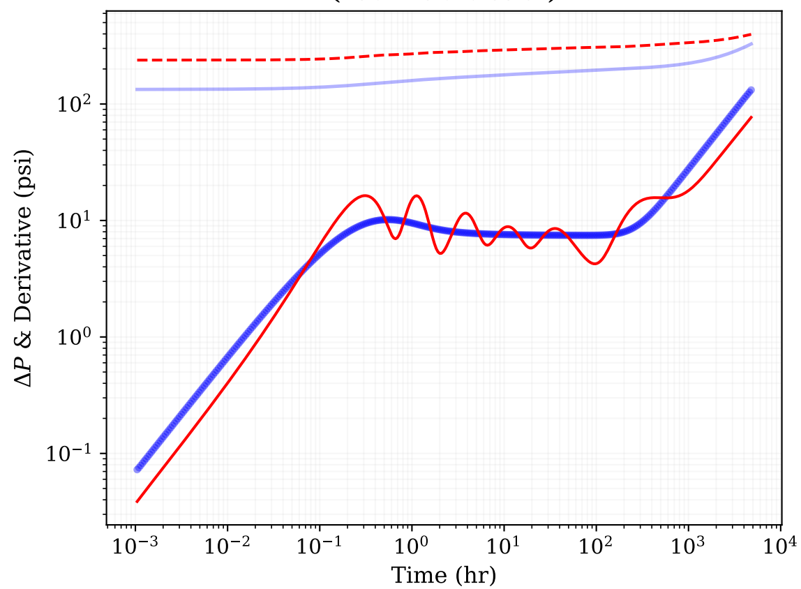
Case: k070_s05_sched1 (Rel. Error: 2.49e-02)
