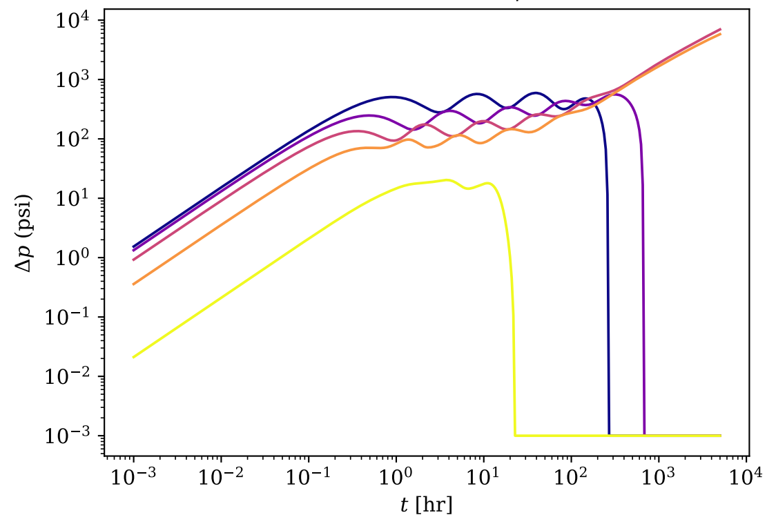
(B) Drawdown \Delta p
