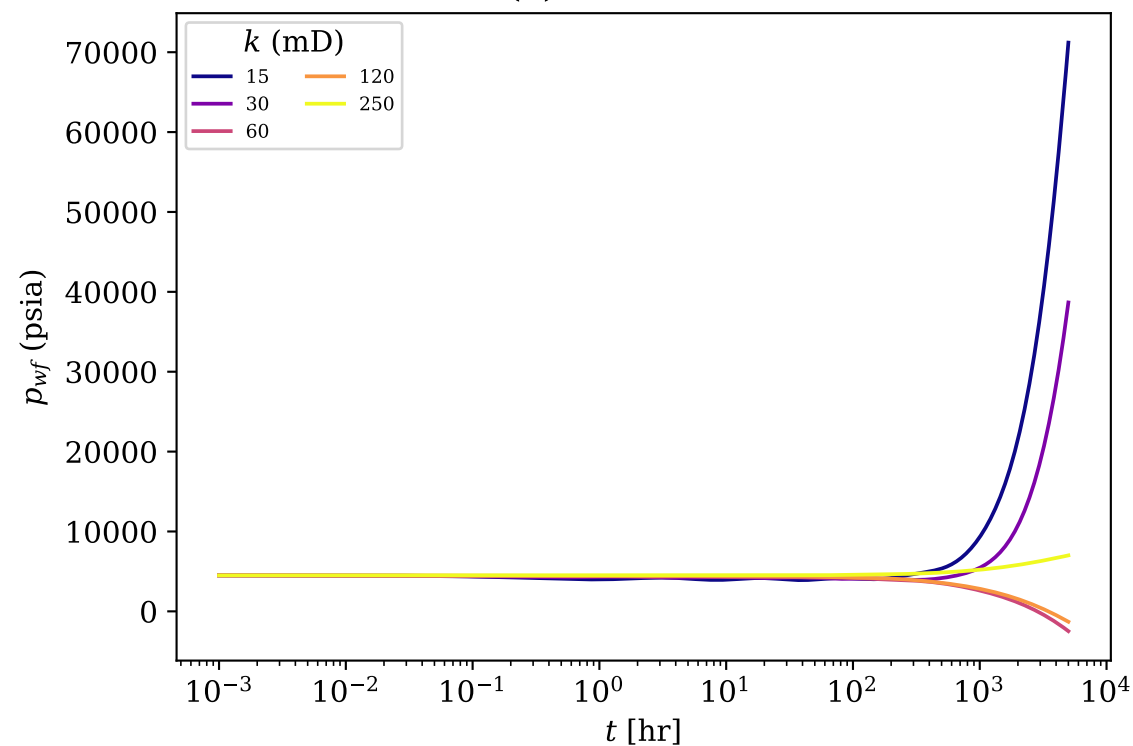
(A) BHP vs time
