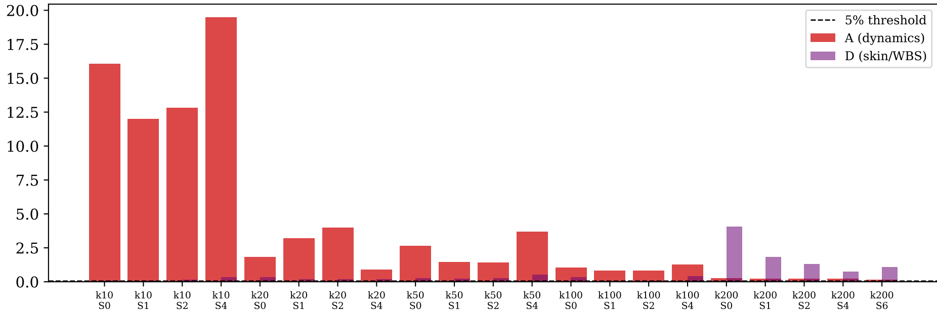
Relative Frobenius error
