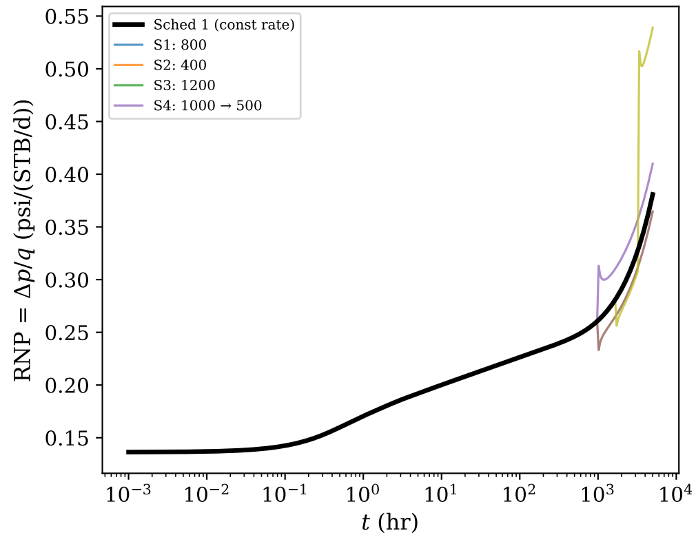
(a) RNP vs real time (schedules spread)
