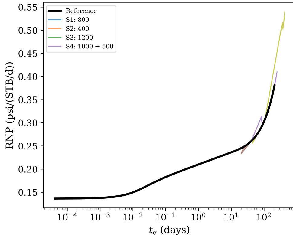
(b) RNP vs t_e (Blasingame collapse)
