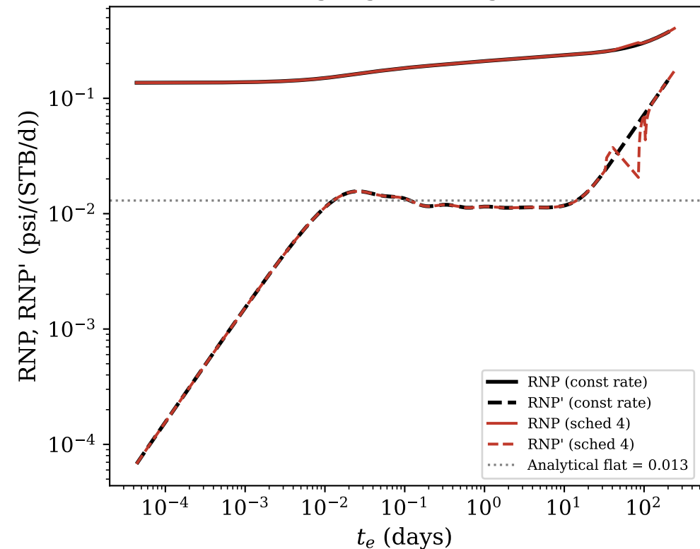
(c) Log-log RTA diagnostic
