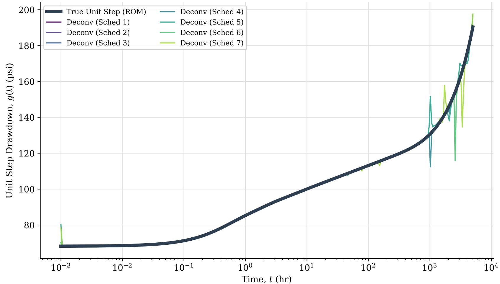
Recovered Pressure Signature
