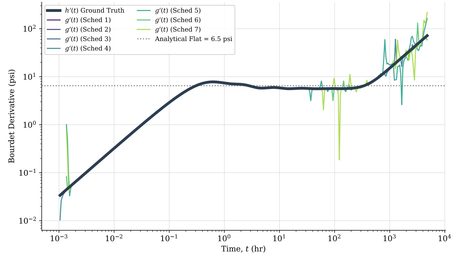
Log-Log Derivative Signature
