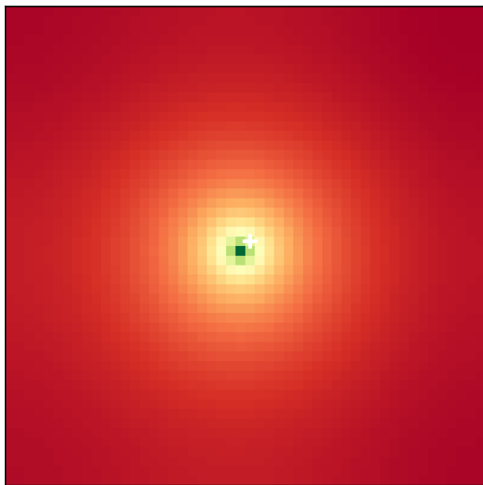
p field, k = 25 mD, t = 2465 hr
