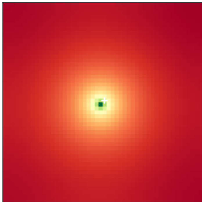
p field, k = 15 mD, t = 2465 hr
