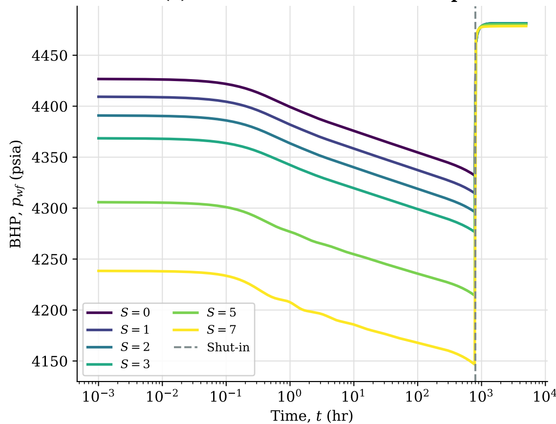
(a) BHP: Drawdown + Build-up
