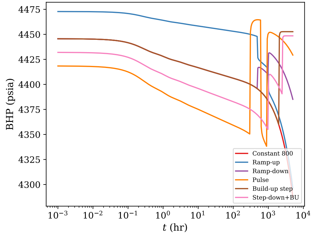
(A) BHP trajectories
