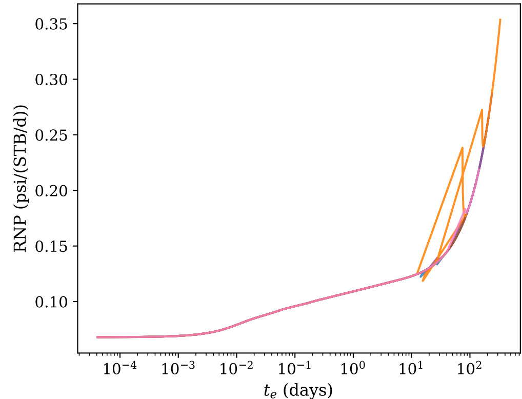
(C) RNP Blasingame — collapse to single curve
