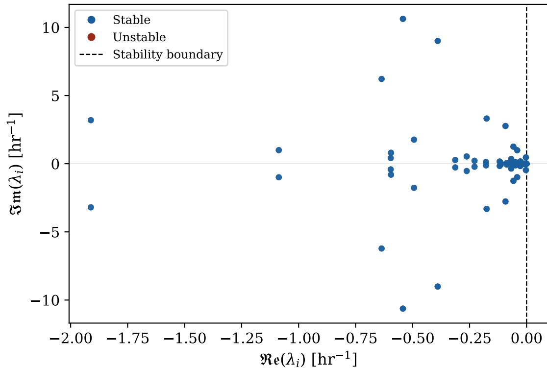
(b) Eigenvalue spectrum of \hat{A}
