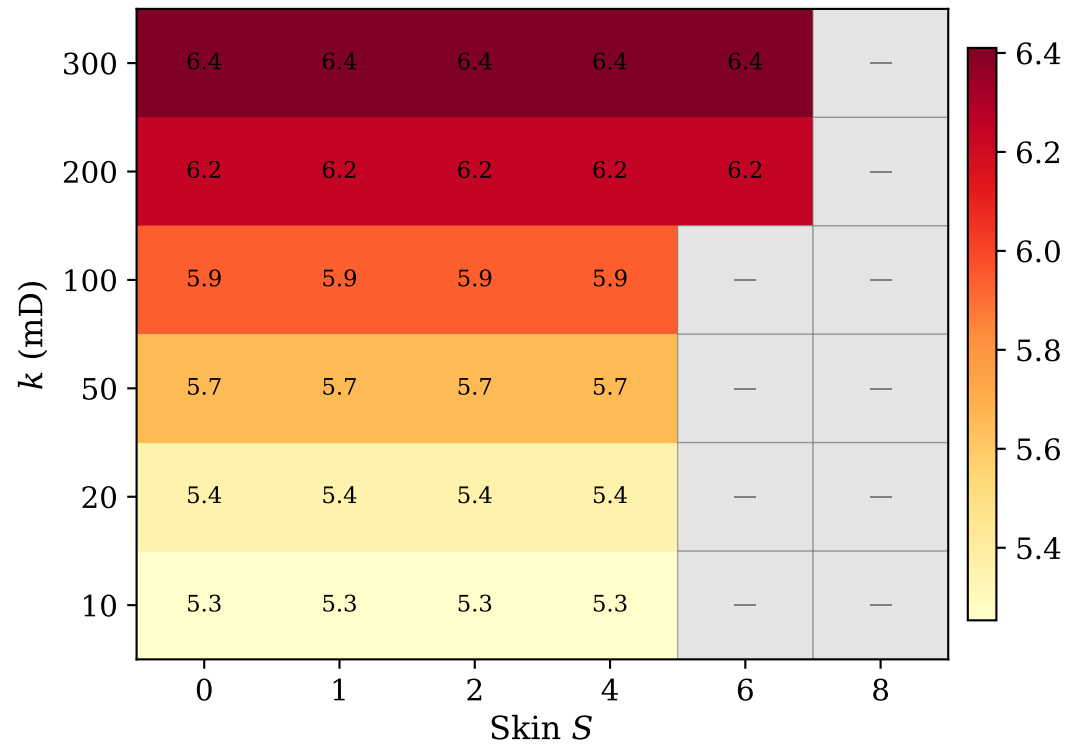
(a) \log_{10} \kappa(\mathbf{D})
